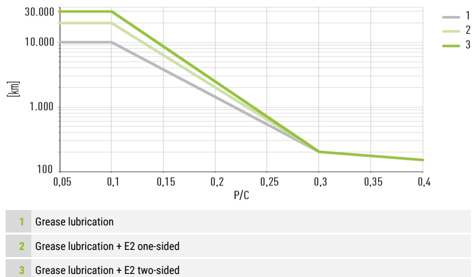
Fig. 8.22: Relubrication intervals with grease lubrication, one-sided and two-sided long-term lubrication unit (E2/EC) for QH, QE and QW. The long-term lubrication unit (E2/EC) is not available for the QW series.
