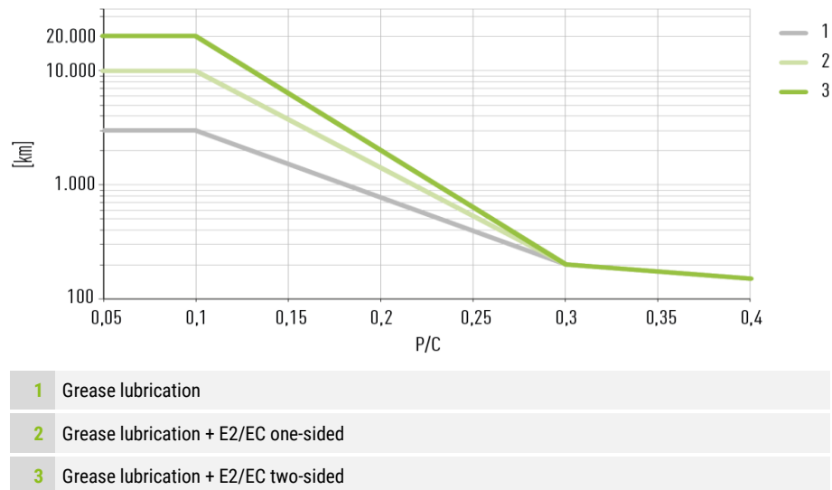
Fig. 8.21: Relubrication intervals with grease lubrication, one-sided and two-sided long-term lubrication unit (E2/EC) for HG, EG, CG, WE. The long-term lubrication unit (E2/EC) is not available for the WE series.
